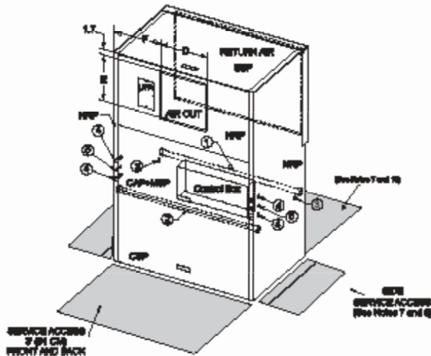
REAR RETURN FRONT DISCHARGE (RRFD)
